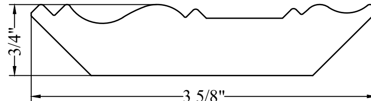
CR0017-00 CR0017-01 3/4" x 3 5/8"
